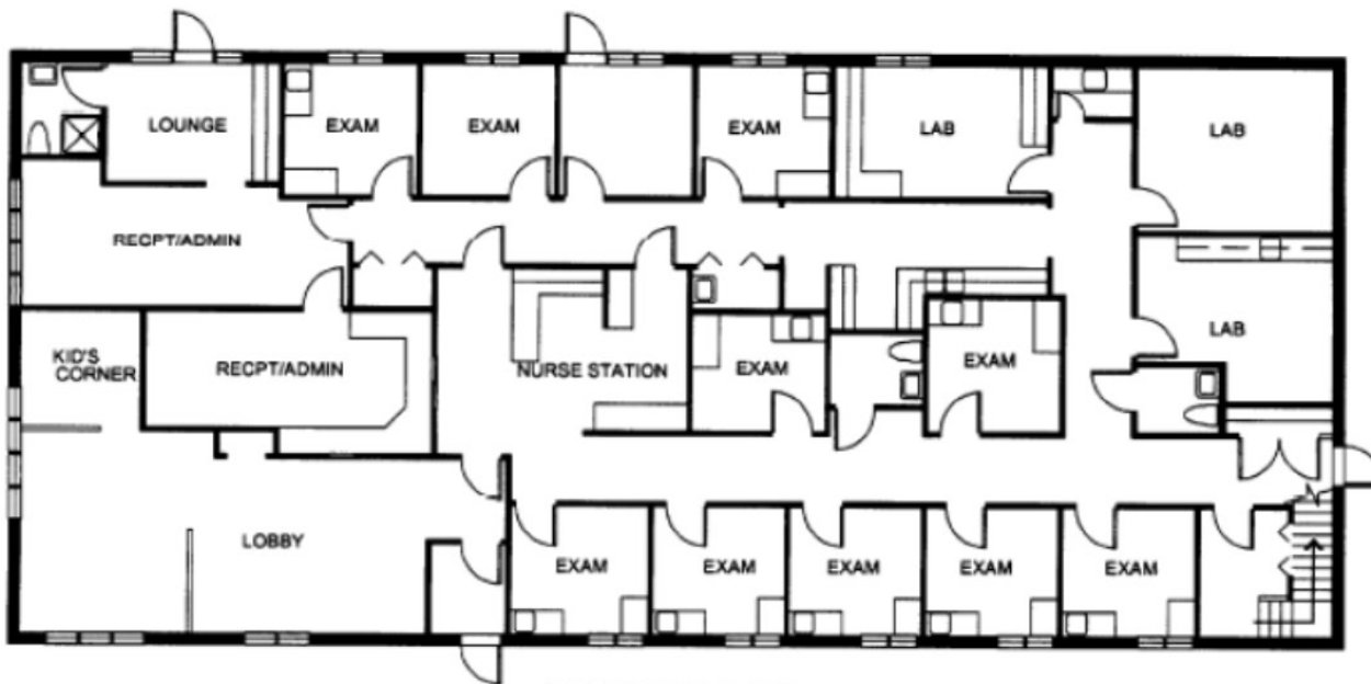
FIRST FLOOR
